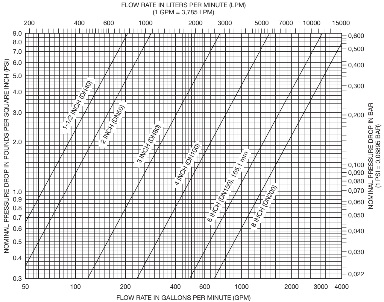
GRAPH A DV-5A VALVE NOMINAL PRESSURE LOSS VERSUS FLOW
