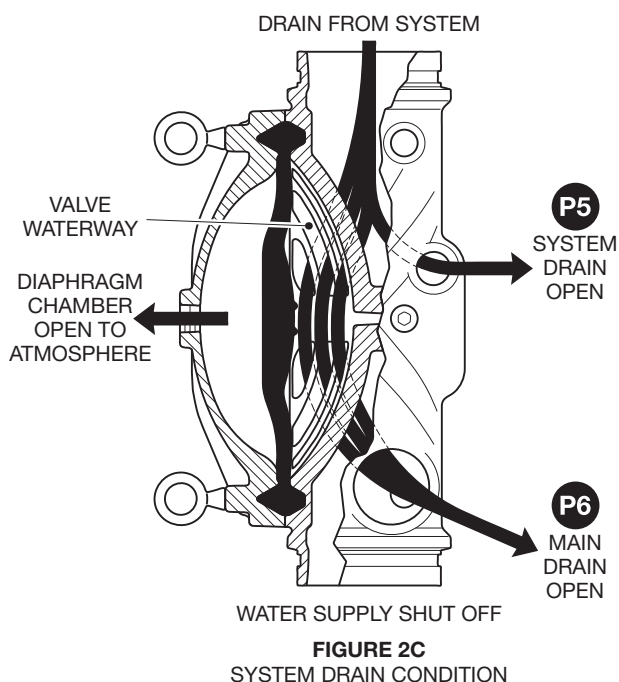
FIGURE 2 DV-5A VALVE OPERATION, DELUGE REMOTE-RESETTING SYSTEMS
